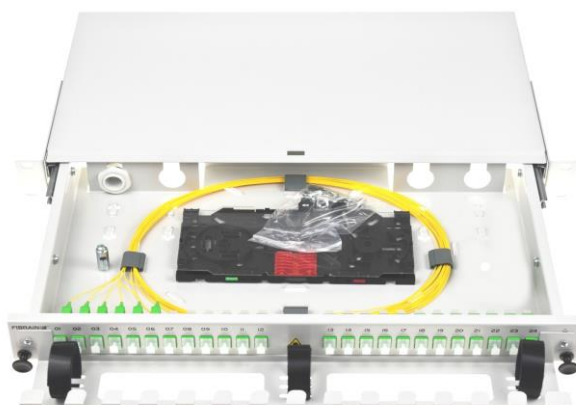
Example of equipped patch panel
