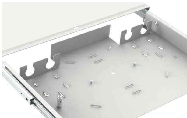
perpendicular cable entries in PST-A1-x type
